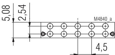
Spring contact block KO 4303-400.1
